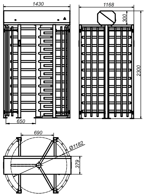
Y-rotor
